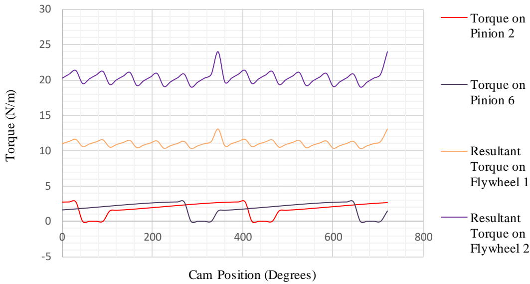
Figure 10 - Torque fluctuation along the pinion gears and flywheels, K = 10000 N/m
