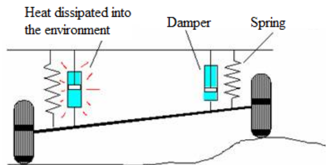
Figure 1 – Heat dissipation in suspension system (Courtney and Klee, n.d)
