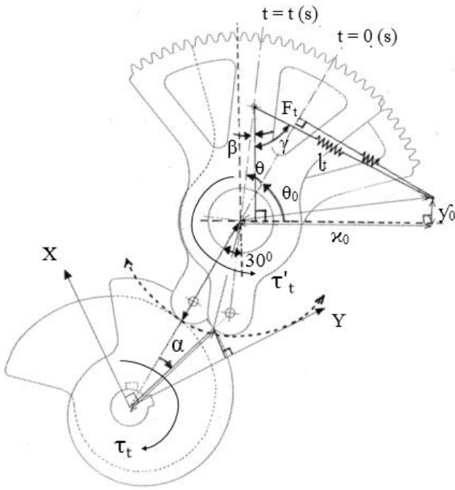
Figure 7 – Schematic diagram used for mathematical model
