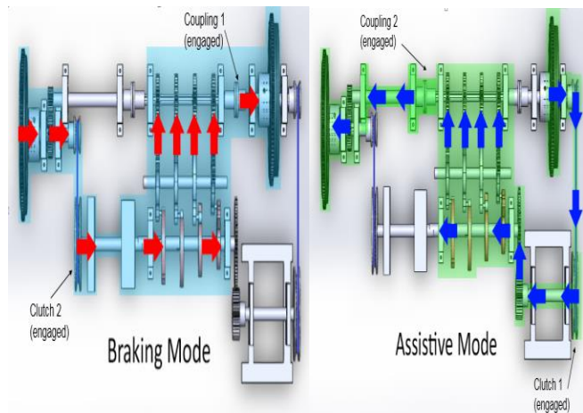
Figure 6 – Power transmission paths
