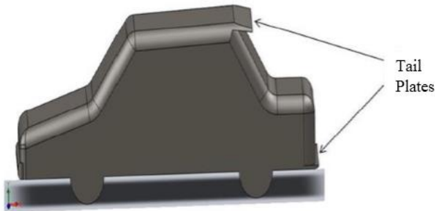
Figure 3 – Passenger car with tail plates (Sharma et al., 2013)
