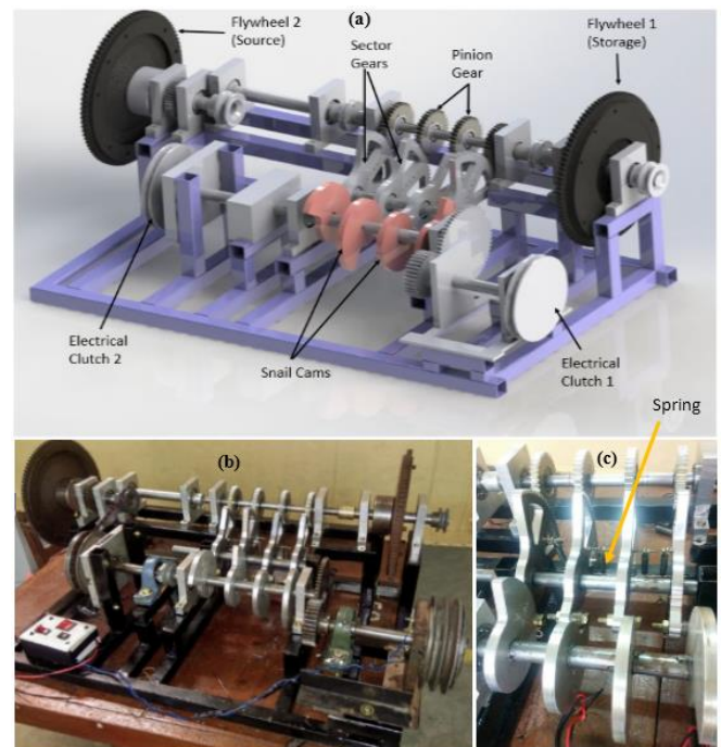
Figure 5 – Secondary stage prototype and 3D model
