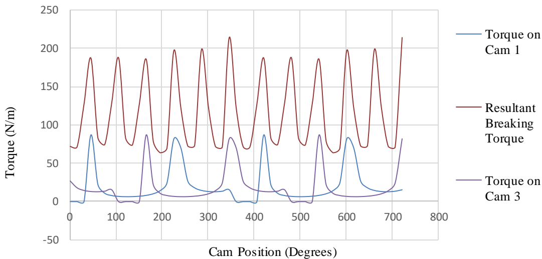
Figure 11 - Torque variation on cams and cam shaft with cam position, K = 10000 N/m
