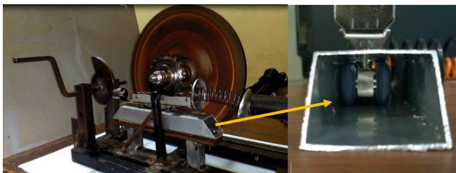
Figure 4 – Primary stage prototype with single snail cam
